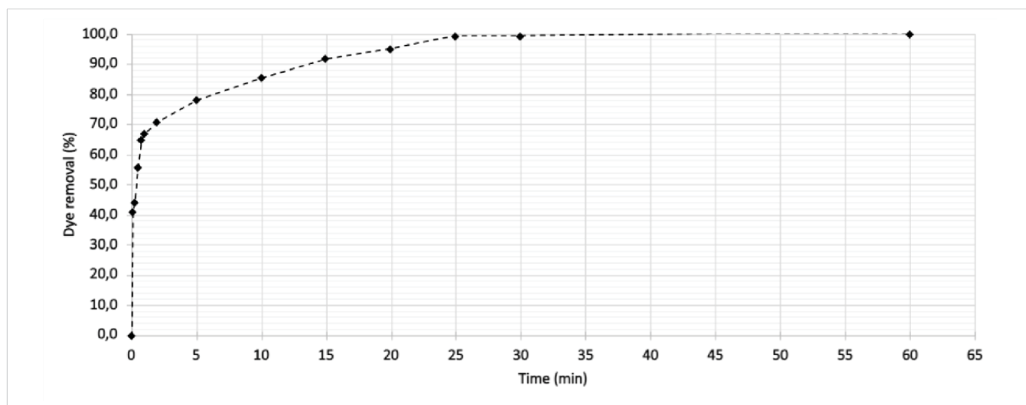
Figure 1: Adsorption kinetics of Reafix B8G yellow dye solution (75 mg.L -1 ) in the presence of boiler ash (0.15 g). The data were obtained keeping the experimental conditions constant, varying only the contact time between the phases.
