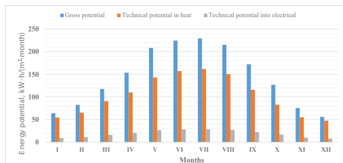
Figure 1: Distribution of the gross and technical potential of solar energy from conversion into thermal and electrical energy in the city of Arkadag by month per 1 square meter during the year.
