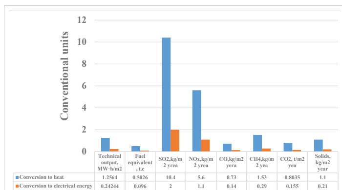
Figure 3: Expected environmental indicators for the reduction of harmful substances into the biosphere of the city of Arkadag from the conversion of solar energy into heat and electricity during the year.
