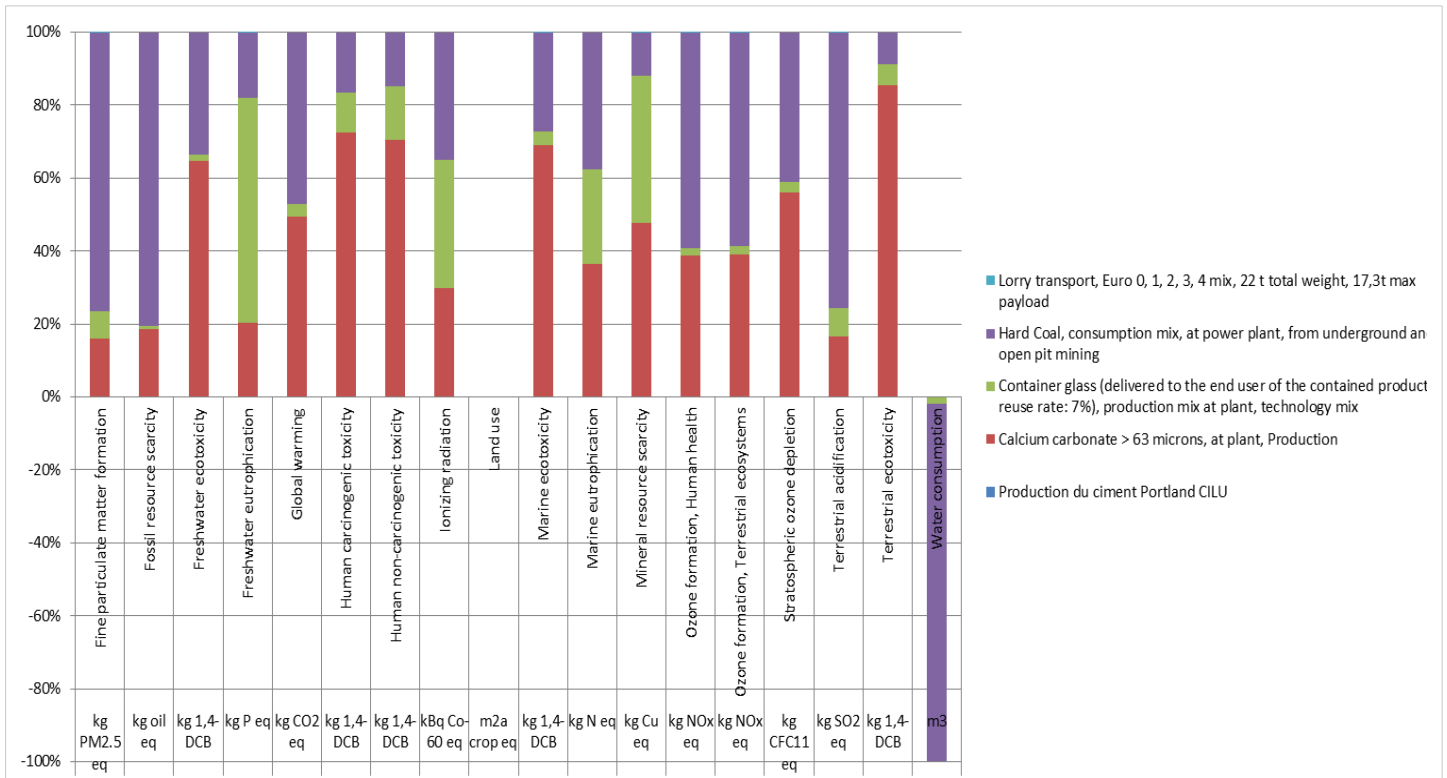
Figure 2: Contribution diagram of the CILU cement manufacturing process in Excel.
