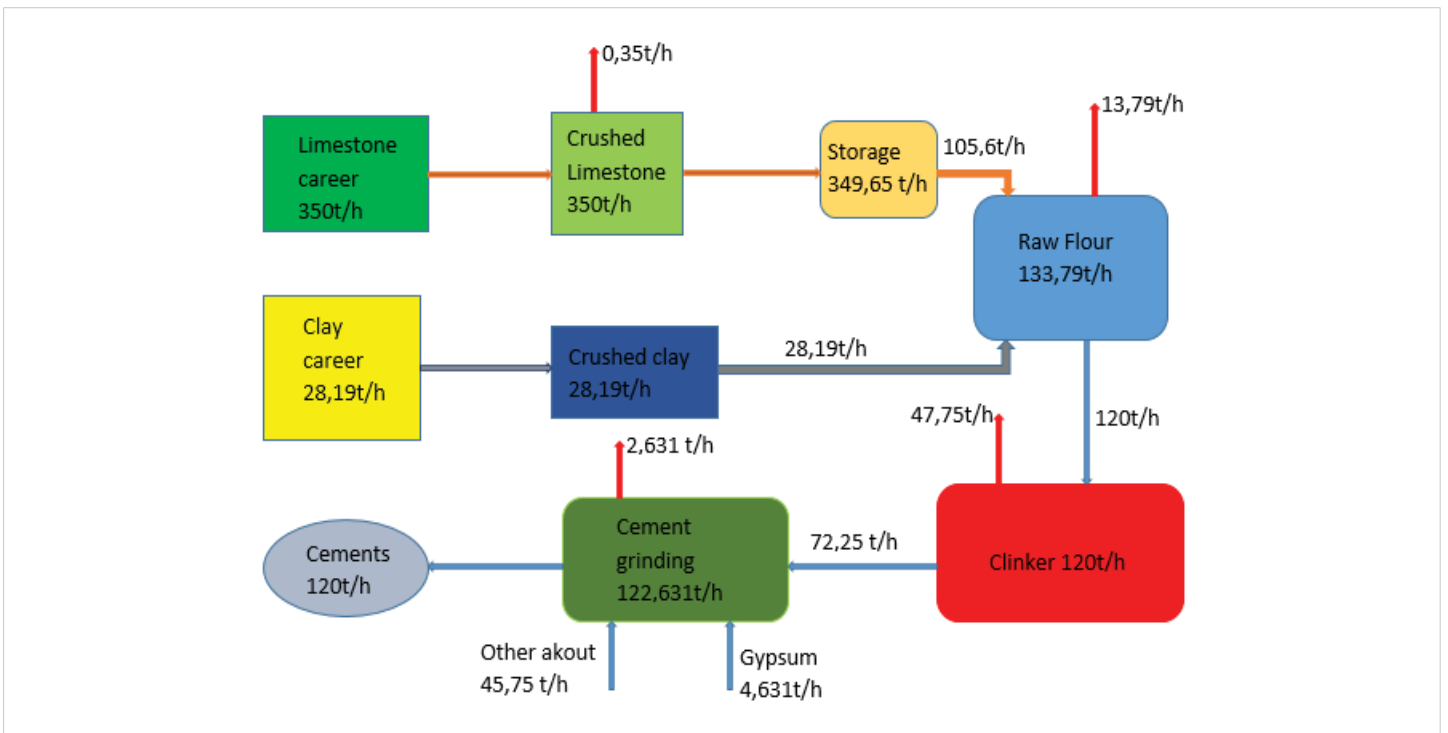
Figure 1: Life Cycle Assessment of the Lukala Cement Plant
